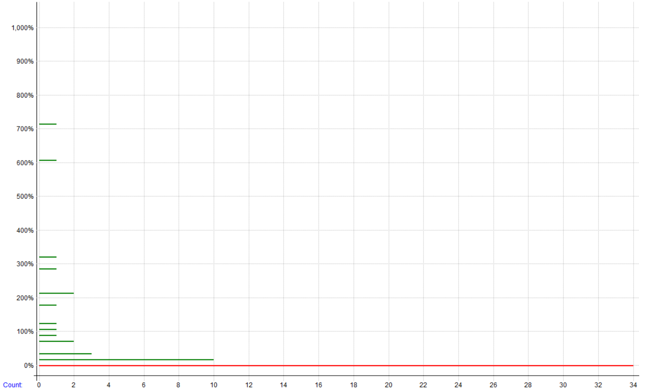
Test 21 - Combined - distribution of %gains
