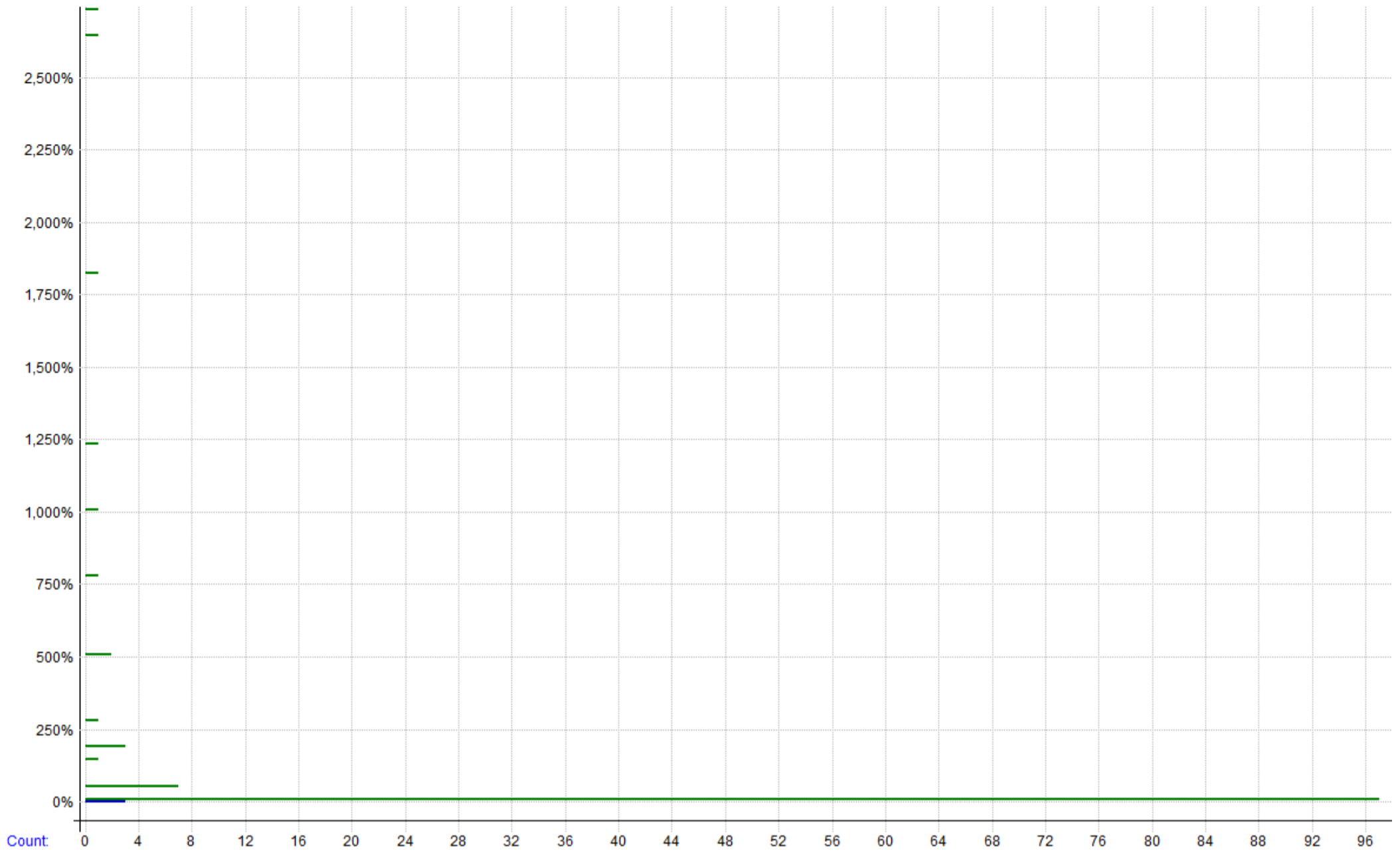
Test 21 - Combined - distribution of %excursions
