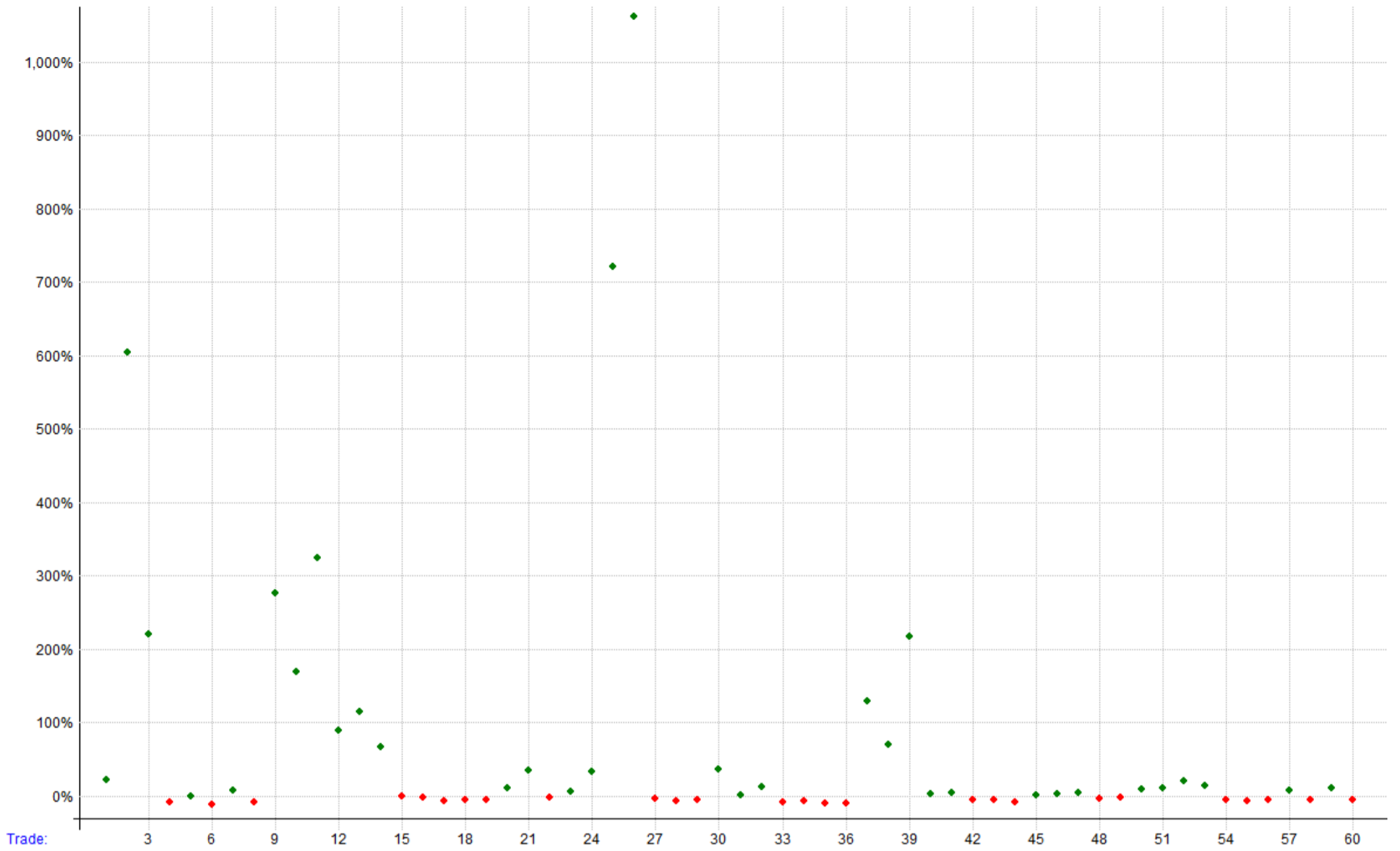
Test 21 - Combined - distribution of %gains
