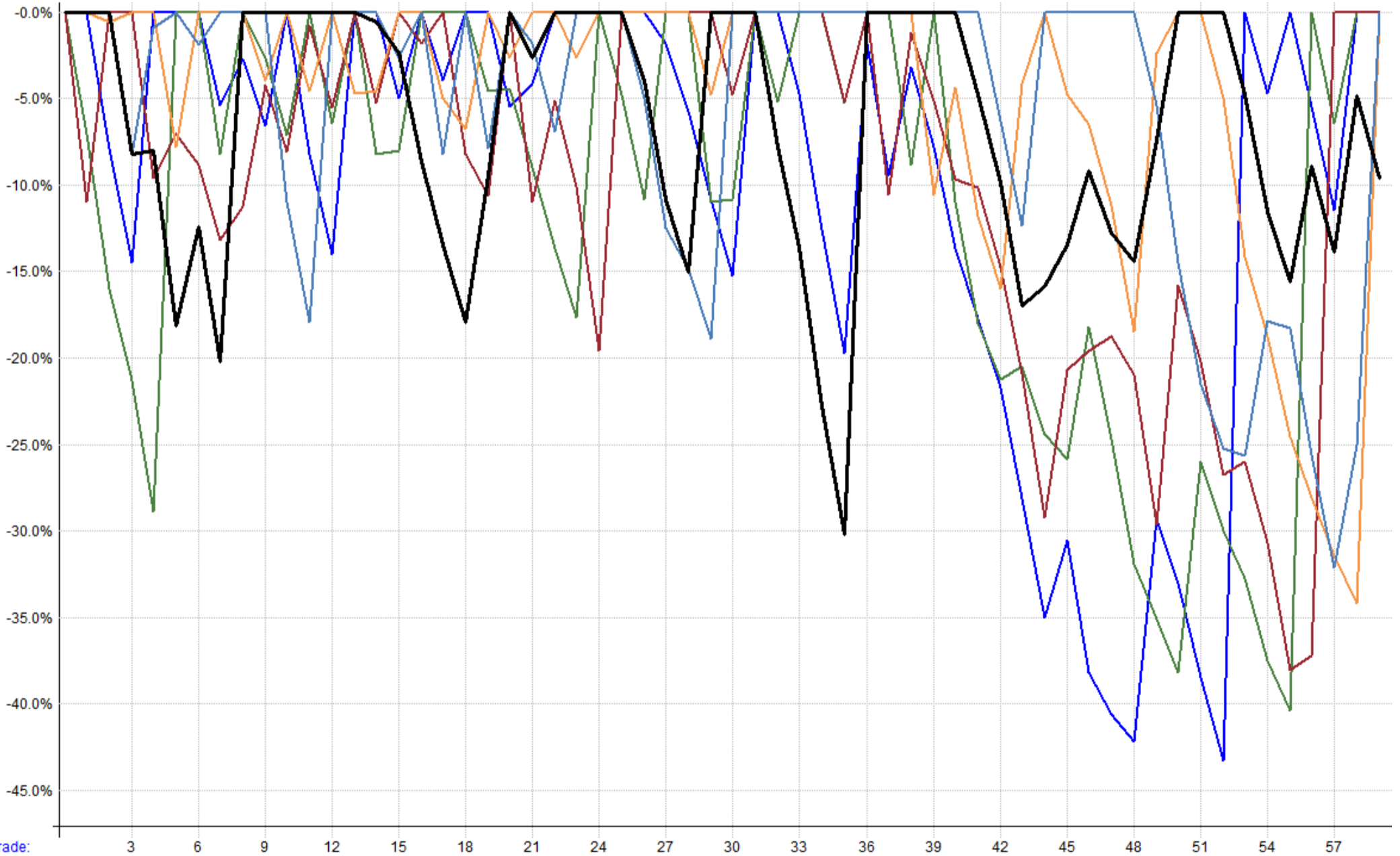
Test 21 - Combined - Monte Carlo %drawdown - 100 samples, showing worst 5
