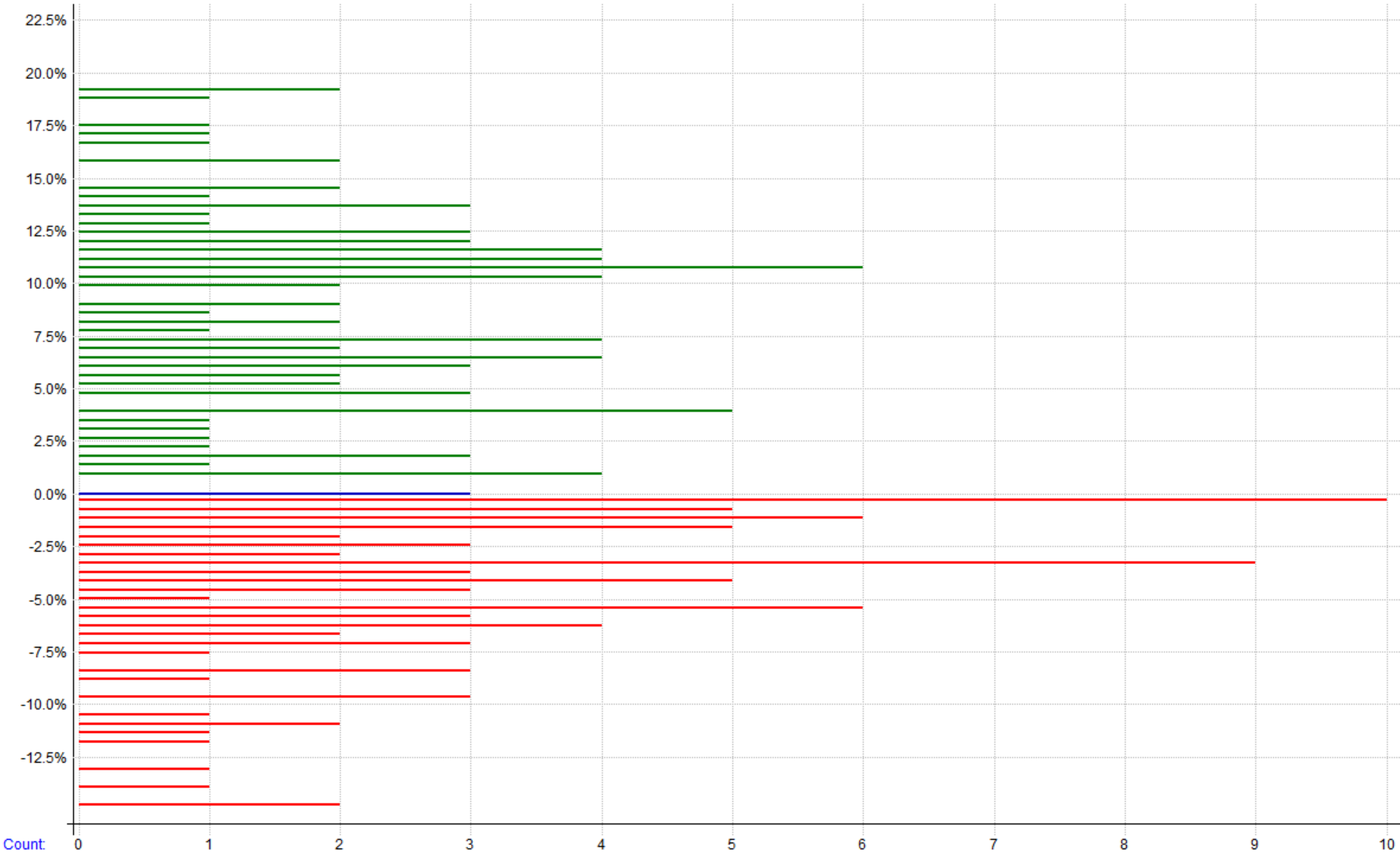
Test 28 - Combined - distribution of %excursions
