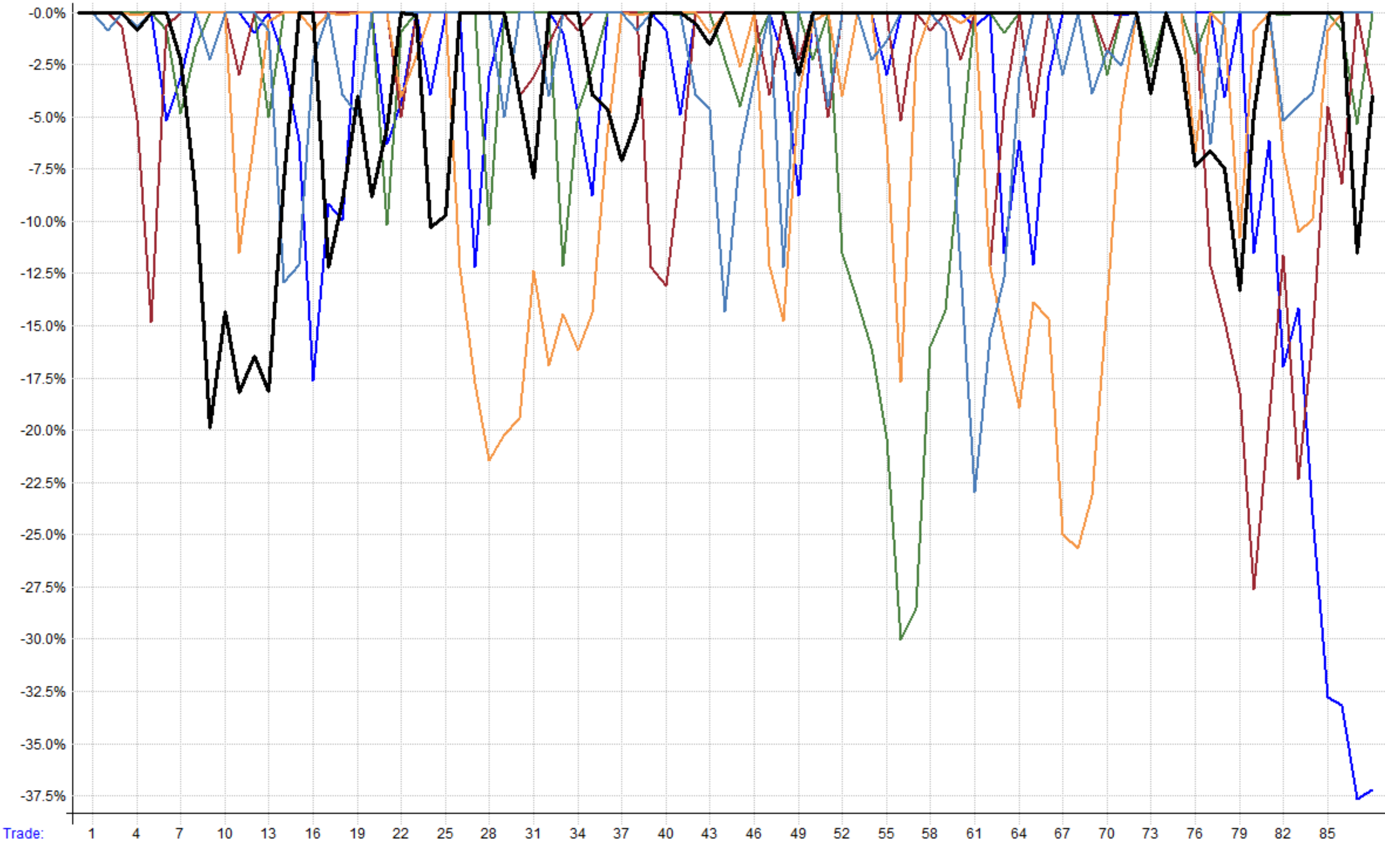
Test 28 - Combined - Monte Carlo %drawdown - 100 samples, showing worst 5
