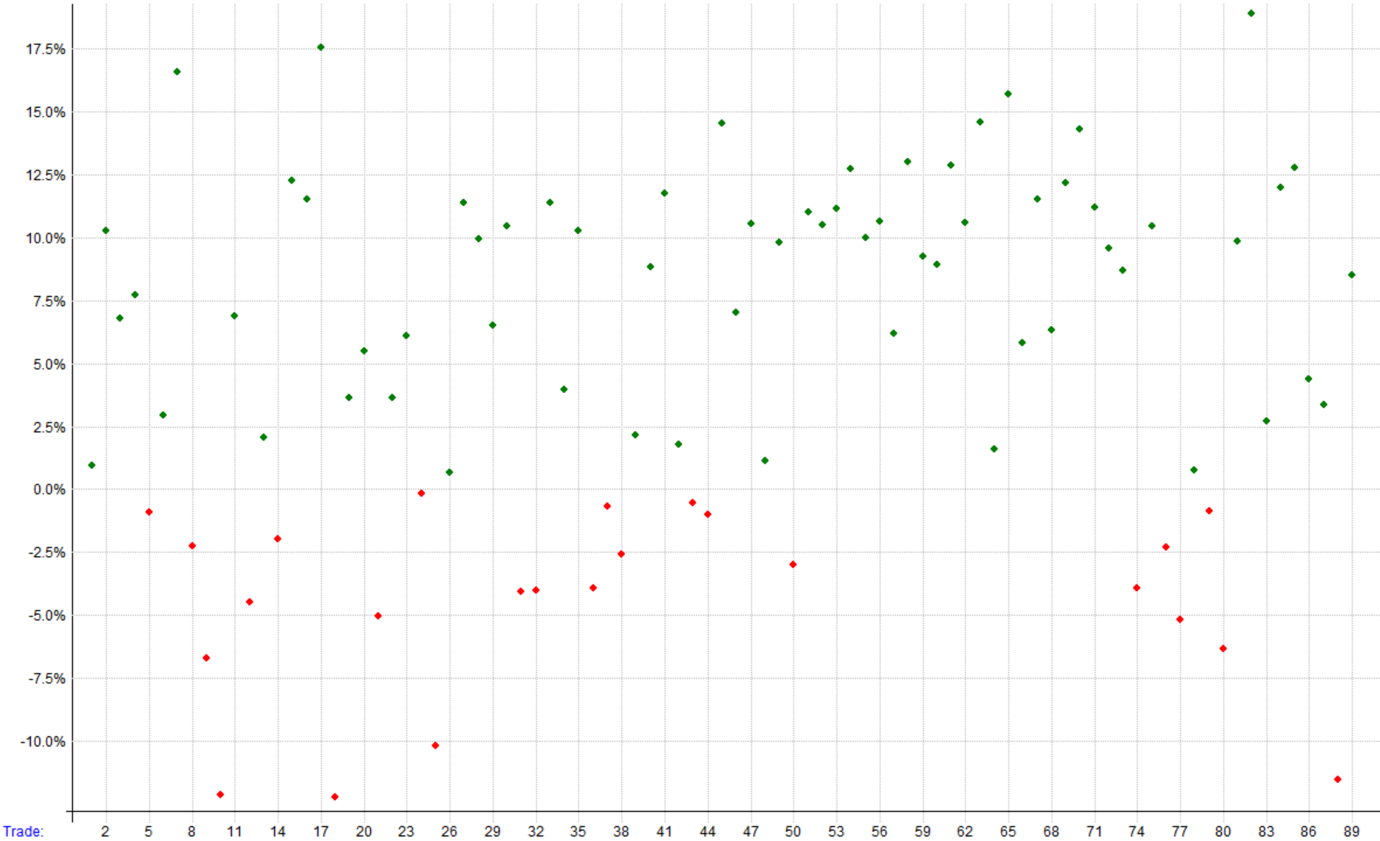
Test 28 - Combined - distribution of %gains
