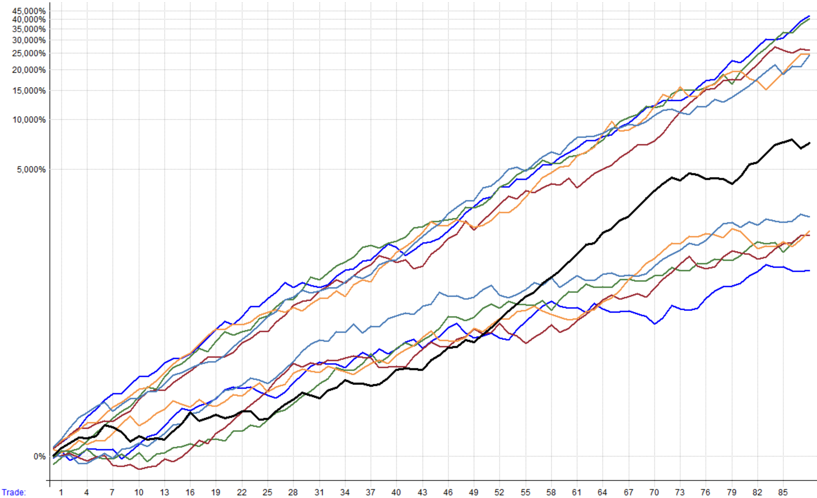
Test 28 - Combined - Monte Carlo %profit - 100 samples, showing best & worst 5
